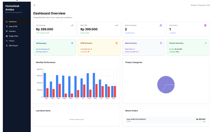
Gambar 10.10 Tampilan Dashboard
