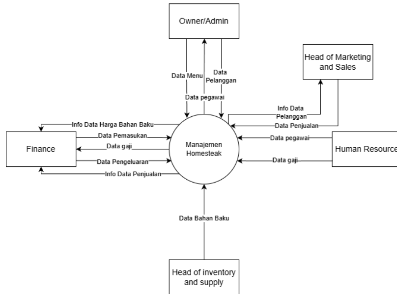
Gambar 4 4. DFD Level 0
