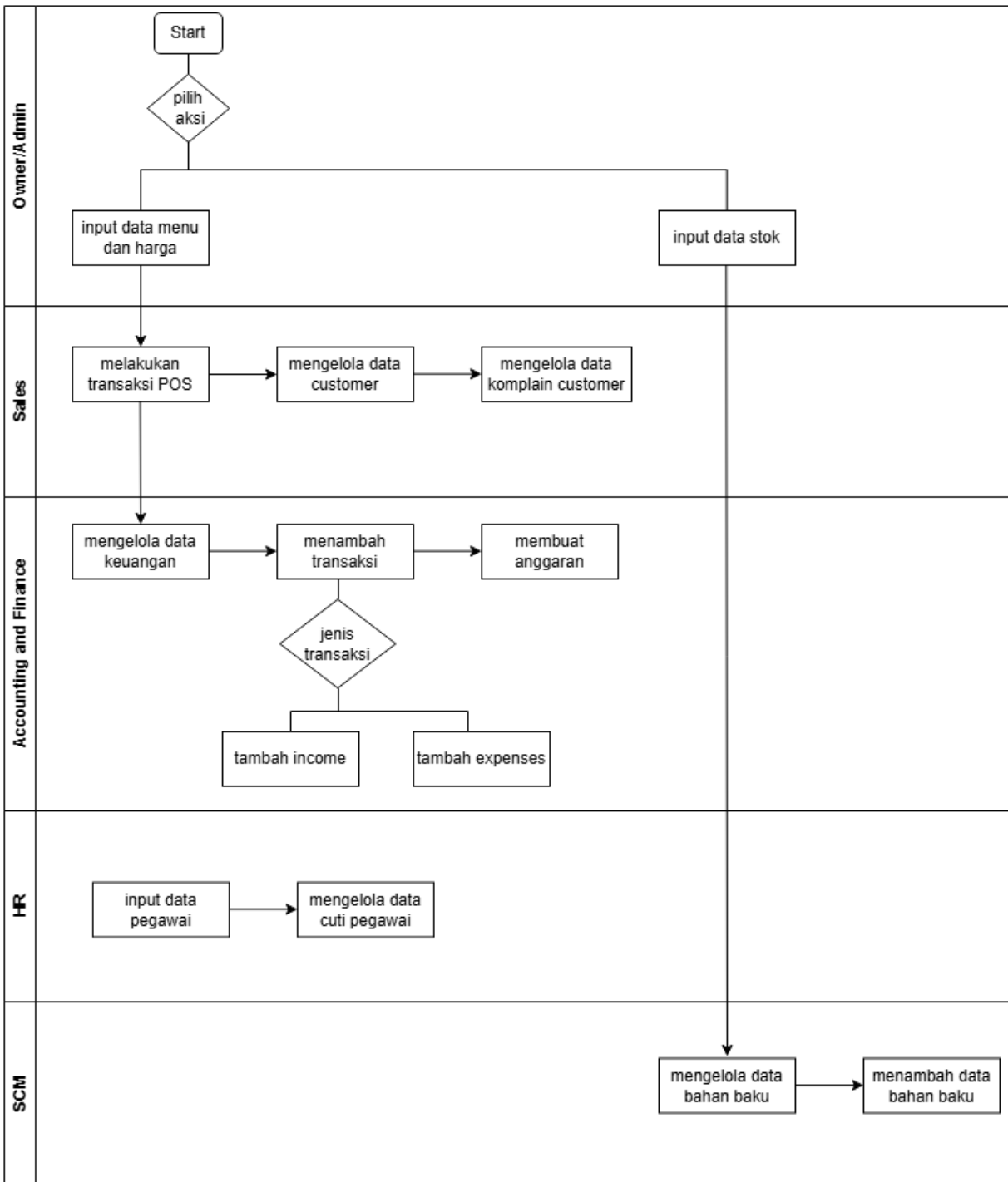
Gambar 3 Swimlane Diagram
