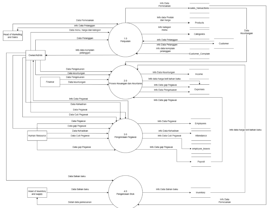
Gambar 55. DFD Level 1
